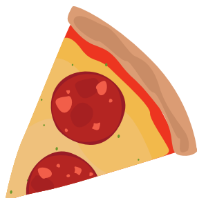
LEFTOVERS
